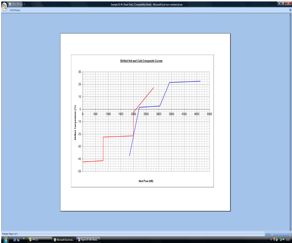
Figure 10-166. A screen-shot of shifted hot and cold composite curves vs. heat flow for Example 10-58.
